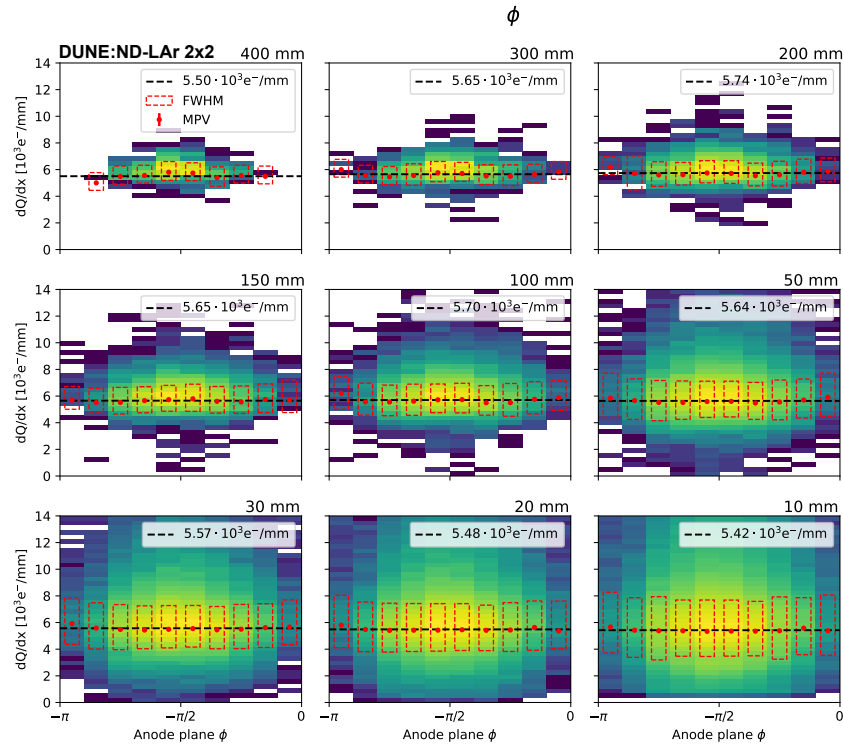
Figure 22. dQ/dx measured for segments of different lengths as a function of the azimuthal angle \phi = \text{atan2}(y, x) , where y and x are the components of the segment along the anode plane axes. The distributions in each bin are fitted with a Gaussian-convolved Moyal function. The red points correspond to the most probable value of the fitted distribution and the dashed rectangles correspond to the FWHM. The dashed black line represents the average MPV.
