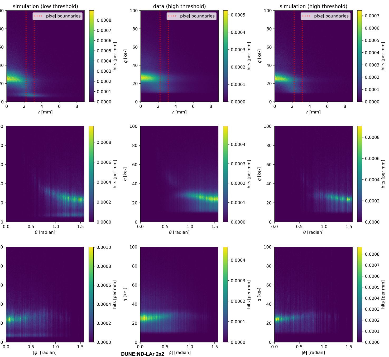
Figure 18. Same as Figure 17 but for high-threshold data.
