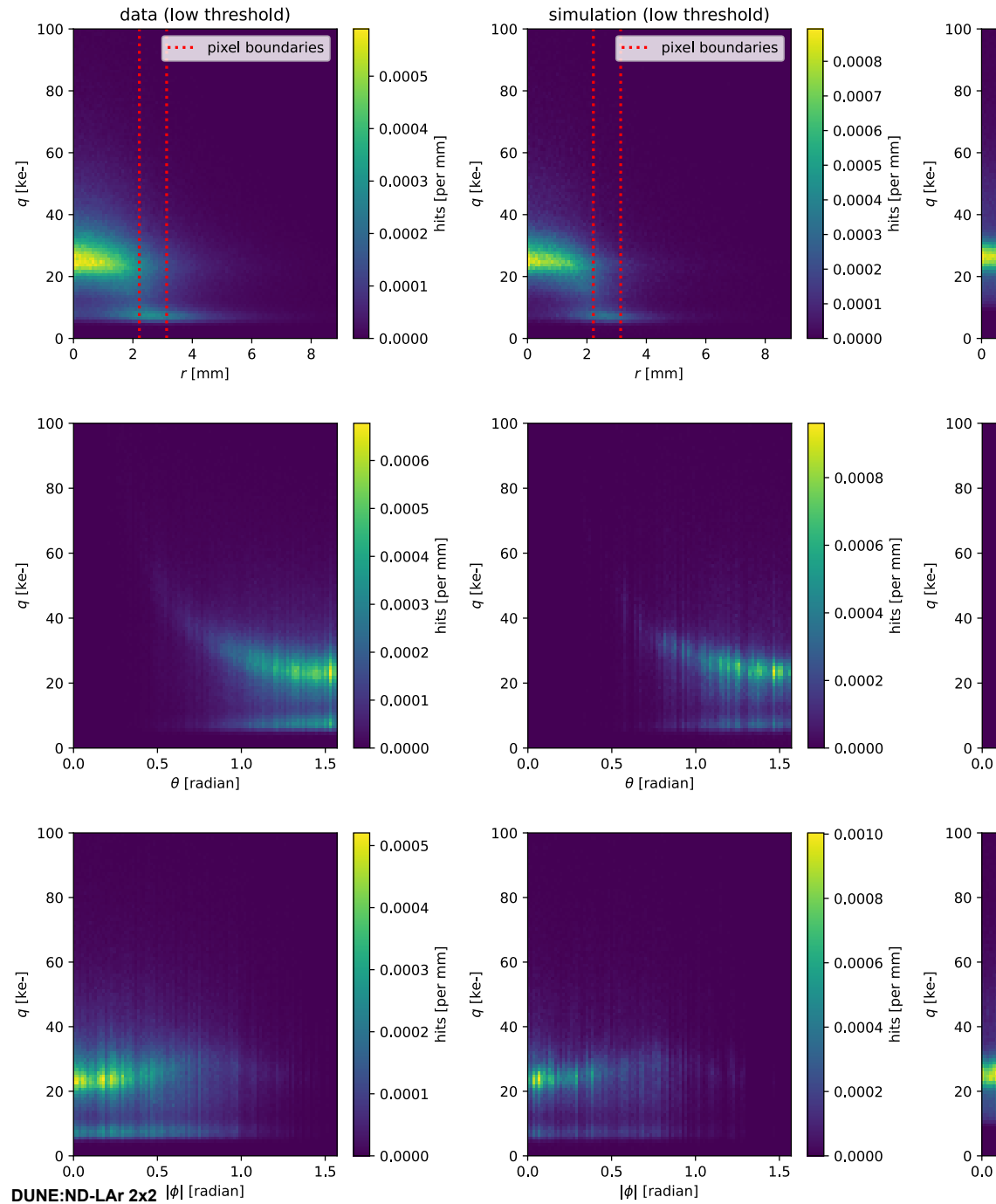
Figure 17. Self-trigger charge distribution for MIP tracks with different track orientations with respect to the pixel, normalized to the number of triggered channels per reconstructed track length. Low-threshold data are used. The MC simulation shown in comparison in the second column is described in Section 5.
