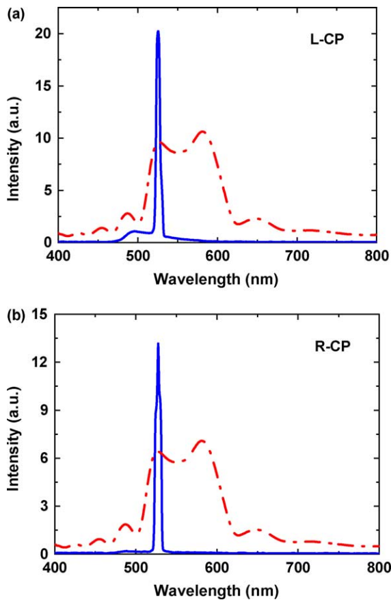
Fig. 5. Lasing emission (solid curve) spectra at the high-energy edge of PBG and reflectance (dash-dot curve) of phase retardation defect mode. (a) L-CP defect mode lasing. (b) R-CP defect mode lasing for the cell with the mixing ratio of chiral NLC polymer of 87 wt% in CLC layers.
