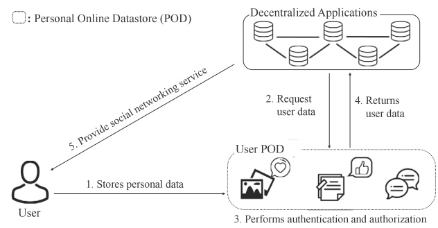
Fig. 3. Solid operations are illustrated with a single POD. A user stores her personal data in her POD, which can be accessed by decentralized social applications depending on the corresponding ACL.
