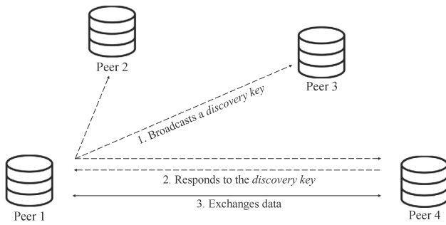
Fig. 5. A flow of the Dat protocol is illustrated. A user discovers peers that hold the object of interest using a discovery key. Then, it exchanges data after negotiating with the peers.
