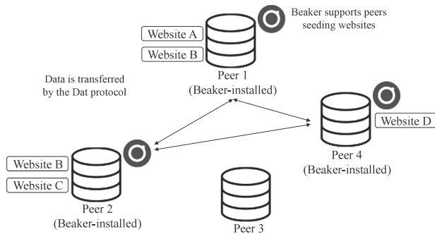
Fig. 6. The operations of Beaker are illustrated. The Beaker browsers running on peers treat a website as a group of files. Thus, websites can be seeded by Beaker-installed peers. The Beaker browser leverages Dat as its underlying exchange protocol.
