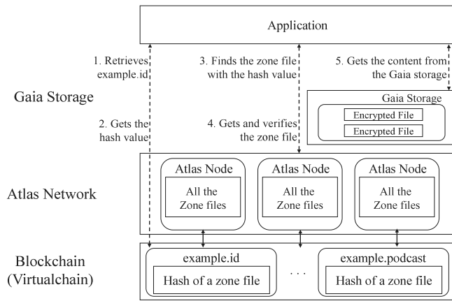
Fig. 8. The operations of Blockstack are illustrated. The blockchain maintains the hash of the zone file of every user (under her name), and the Atlas network contains the zone file, which includes the location of the user's data locker in Gaia.
