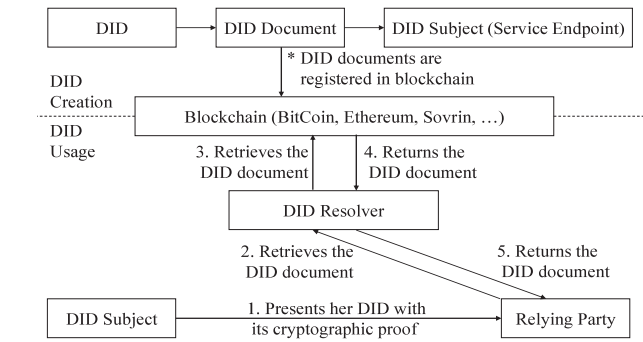
Fig. 10. The operations of how a subject authenticates herself in DIDs are illustrated. First, the subject who wants to prove her identifier sends her DID with a cryptographic proof. Then, the relying party that receives the DID sends a query to the DID resolver and verifies the proof with the DID document in the response.
