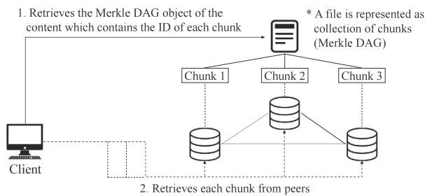
Fig. 1. In IPFS, a file is divided into smaller chunks, and these chunks are aggregated to the original file using the Merkle DAG. The user first requests the file then receives its chunk IDs. Finally, the user requests each chunk by its chunk ID.
