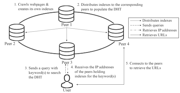
Fig. 7. The operations of YaCy are illustrated. Each peer crawls websites and makes its own indexes, which populate the DHT for keywords. When a user sends a query, YaCy looks up its DHT to find out the IP addresses of the peers (that hold the relevant URLs in their indexes). Finally, the user connects to the peers to retrieve the URLs.
