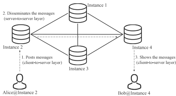
Fig. 4. The operation of Mastodon is illustrated. A user registers her account with the Mastodon instance, where the combination of the username and the instance is globally unique. Therefore, each user is identified by her name, by which message exchanges between users occur.
