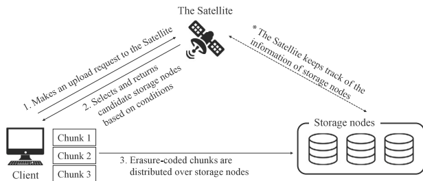
Fig. 2. Data uploading operations in Storj are illustrated. Thanks to the Satellite and the erasure coding, Storj can enhance its delay performance and availability compared to IPFS.
