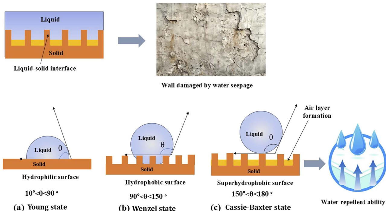
Fig. 5 Diagram illustrating various surface wettability through contact angle measurements.
