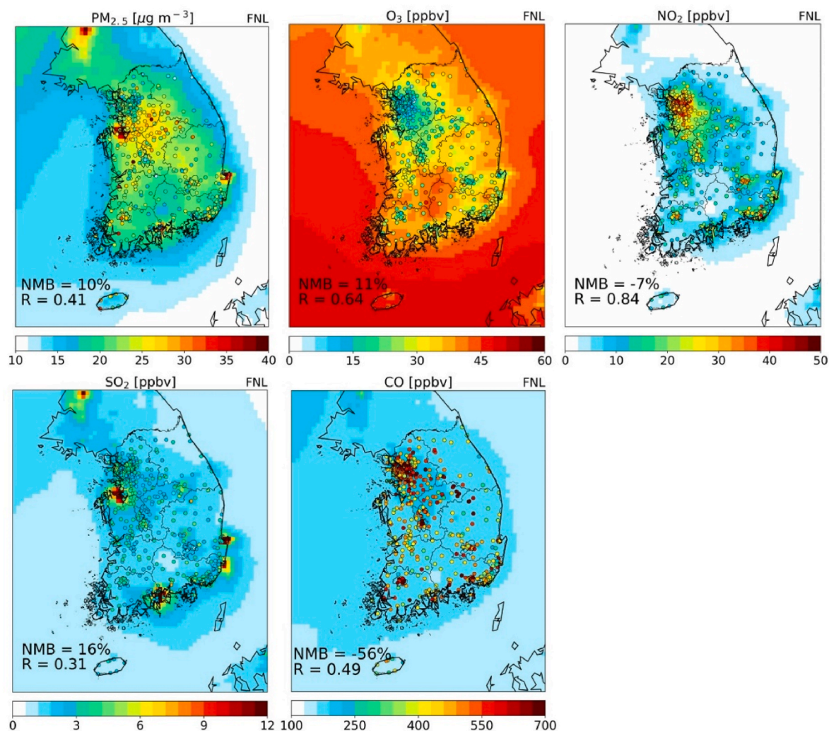
Fig. 4. A model ensemble obtained using FNL meteorological input fields and observed mean values of PM_{2.5} , O_3 , NO_2 , SO_2 , and CO surface concentration during the GMAP campaign (October 18 to November 25, 2021). The background represents model values, and circles indicate the location of 505 Air-Korea surface monitoring stations and their observed values.
