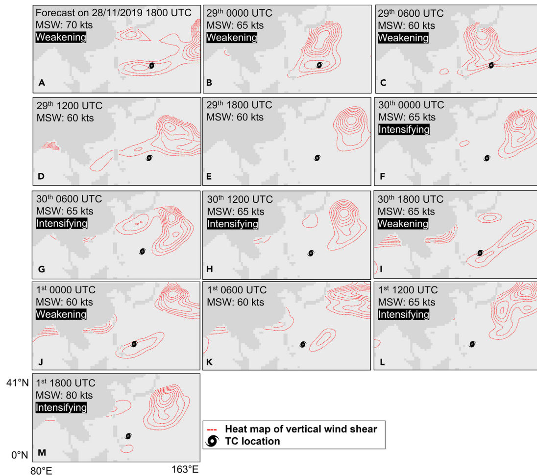
Figure 7. Heatmaps of vertical wind shear (red contour) over typhoon KAMMURI (72-h forecasting for 01/12/2019 1800 UTC)
