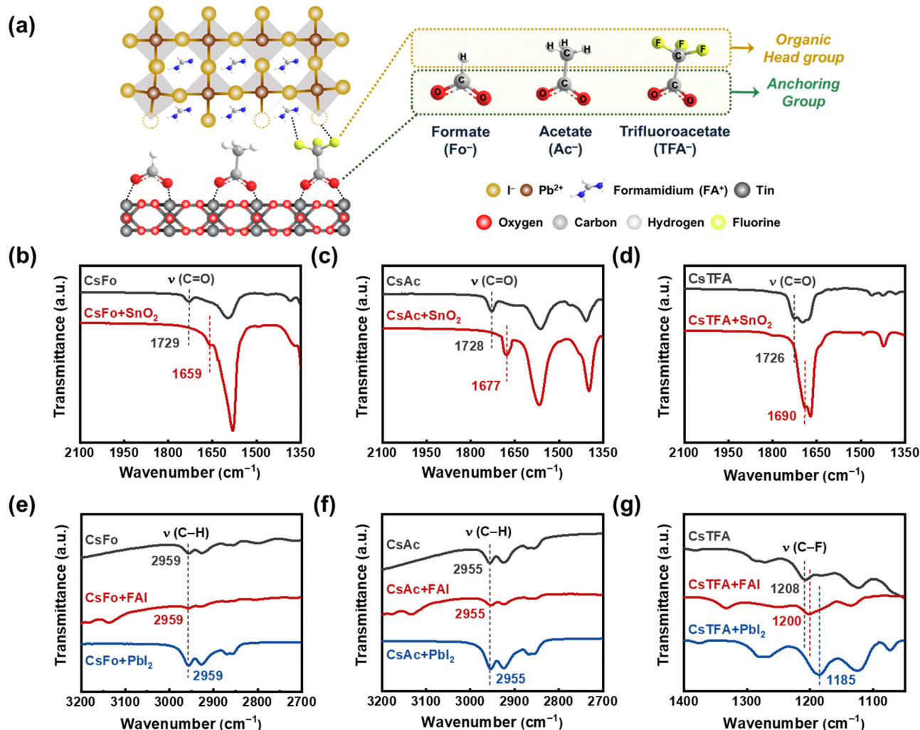
Fig. 1 (a) Schematic illustration of the CsX ( X = \text{Fo}^- , \text{Ac}^- , and \text{TFA}^- ) treatment process applied to the \text{SnO}_2 ETL. FTIR spectra of CsX, CsX-SnO 2 , CsX-FAI, and CsX-PbI 2 , (b) and (e) CsFo, (c) and (f) CsAc, and (d) and (g) CsTFA.
