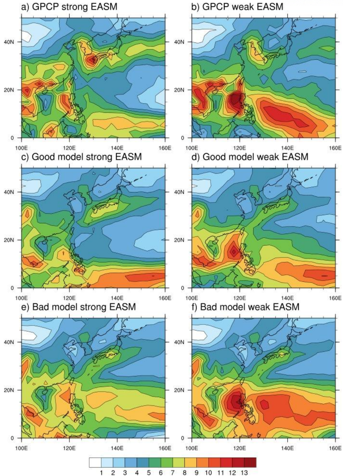
Figure 3.6. Seasonal mean (JJA) precipitation over East Asia during the summer in (a) GPCP observation strong EASM years, (b) GPCP observation weak EASM years, (c) good models strong EASM years, (d) good models weak EASM years, (e) bad models strong EASM years and (f) bad models weak EASM years.
