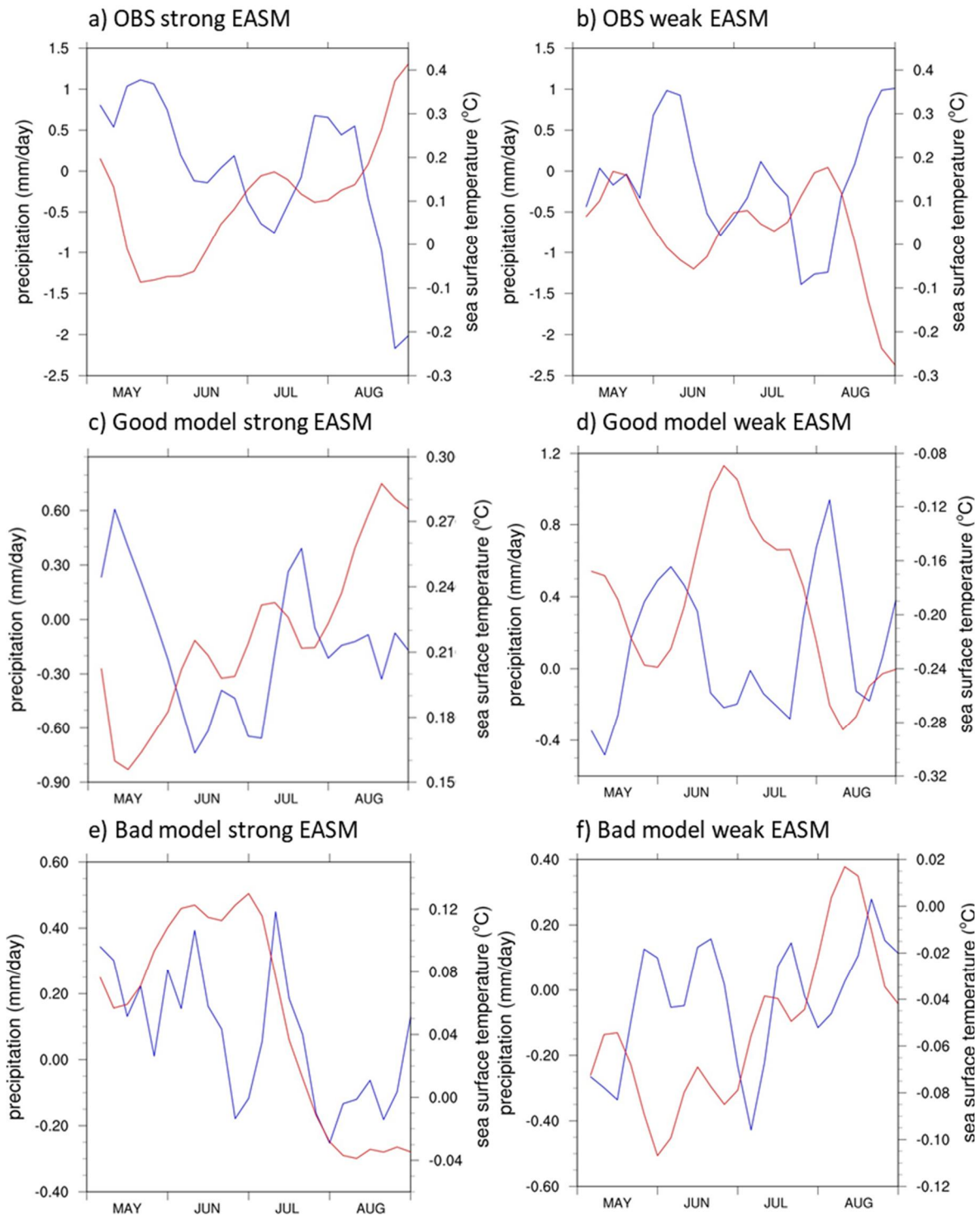
Figure 3.8. Time series of precipitation anomaly (mm·day -1 ) and SST anomaly (°C) over 20-30°N, 120-140°E in (a) observation strong EASM years, (b) observation weak EASM years, (c) good model ensemble strong EASM years, (d) good model ensemble weak EASM years, (e) bad model ensemble Strong EASM years, and (f) bad model ensemble weak EASM years.
