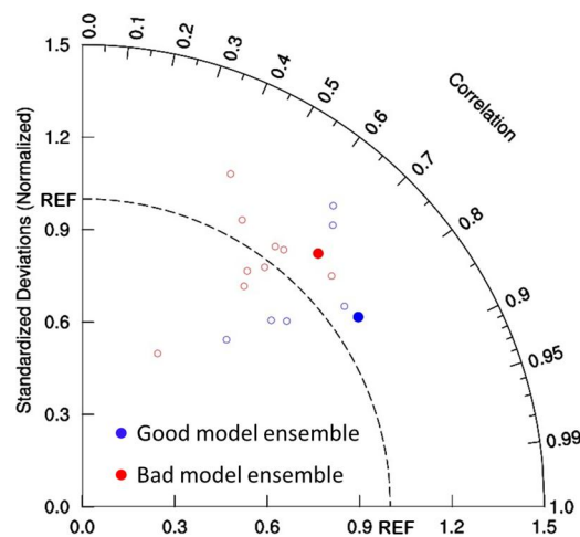
Figure 3.1. Pattern correlation and spatial standardized deviation of ratio for the seasonal (JJA) mean precipitation between observation and CMIP5 good models and (blue) and CMIP5 bad models (red) for 27 years (1979-2005).
