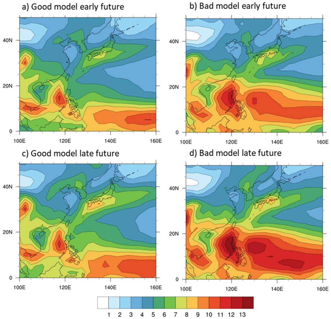
Figure 3.11. Seasonal mean (JJA) daily precipitation ( \text{mm day}^{-1} ) over East Asia of (a) good models in early future (2020-2049), (b) bad models in early future, (c) good models in late future (2070-2099), and (d) bad models in late future.
