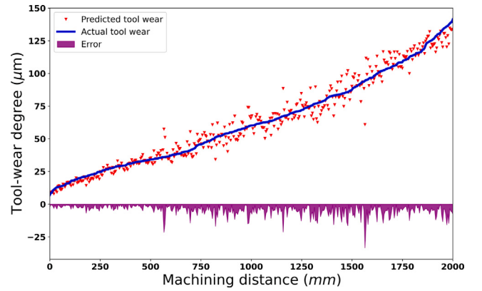
Fig. 11. Prediction results of DMSCNN on Dataset 3.
