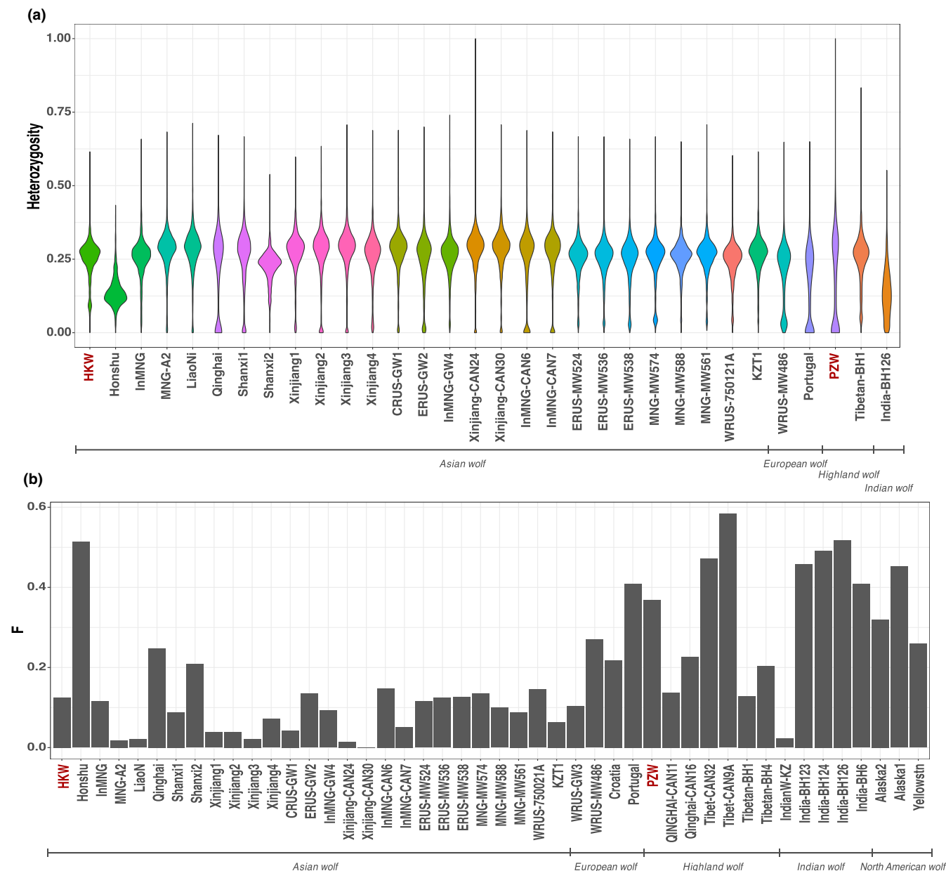
FIGURE 4 Assessing HKW genetic diversity. (a) Heterozygosity estimated in 1Mb genomic windows for Asian wolves and representative European, Indian and Highland wolves. The HKW displays similar heterozygosity to most of the compared wolf individuals, but it shows a proportion of low heterozygosity regions. (b) Inbreeding coefficients ( F ) estimated for all modern and historical wolves in our dataset. HKW has a low inbreeding value (0.12) when compared to the rest of the wolf samples. Both analyses were performed on genotype imputed data. HKW, historical Korean wolf.
