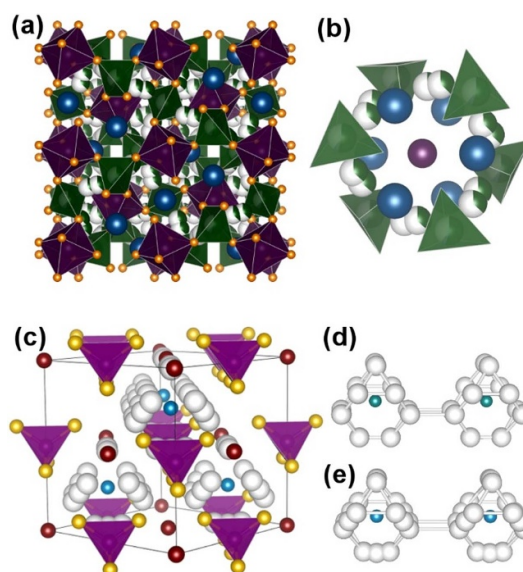
Figure 14. Crystal structure representations of (a), (b) Al-doped LLZO garnet and (c–e) \text{Li}_6\text{PS}_5\text{X} ( \text{X} = \text{Cl}, \text{Br} ) solid state electrolytes. The cubic phase garnet in (a) is represented by Zr ions (purple, with polyhedra shown), La ions in blue, lithium ions in green, and oxygen in orange. (b) shows the distribution of lithium ions in tetrahedral (polyhedra shown) and distorted octahedral positions in the cubic garnet framework, viewed along the [110] direction. The argyrodite phase \text{Li}_6\text{PS}_5\text{Br} is shown in (c), where white spheres represent lithium ions, yellow represent sulphur, purple spheres are phosphorus ions, maroon spheres represent 4a sites where Br/S anion site disorder is observed, and blue spheres represent 4d disordered Br/S sites. The lithium site disorder for the \text{Li}_6\text{PS}_5\text{Br} phase is shown in (e), in contrast to the chloride analogue (d) where lithium is found only on the 48 h site.
