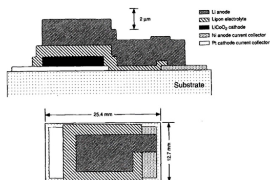
Figure 20. Schematic cross-sectional (top) and plan view (bottom) drawings of a Li/LiPON/LCO thin-film cell. Reprinted with permission from [4]. Copyright 1996, The Electrochemical Society.
