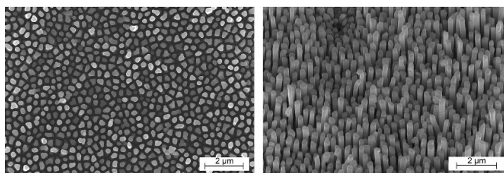
Figure 21. Top view (left) and side view (right) SEM micrographs of aluminium nanorods synthesised by pulsed electrodeposition through an alumina template which was subsequently dissolved away. Adapted with permission from [10]. Copyright (2009) American Chemical Society.
