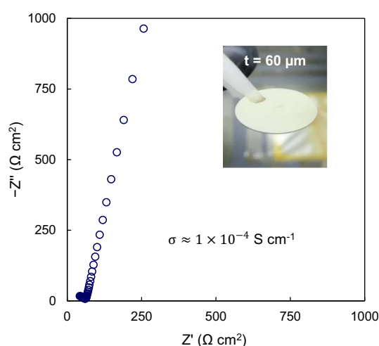
Figure 17. Nyquist plot taken from a 60 \mu\text{m} thick Li 6 PS 5 Cl film comprising 30 individually spray deposited and re-precipitated layers, measured between two stainless-steel spacers under a uniaxial clamping stress of 400 MPa.
