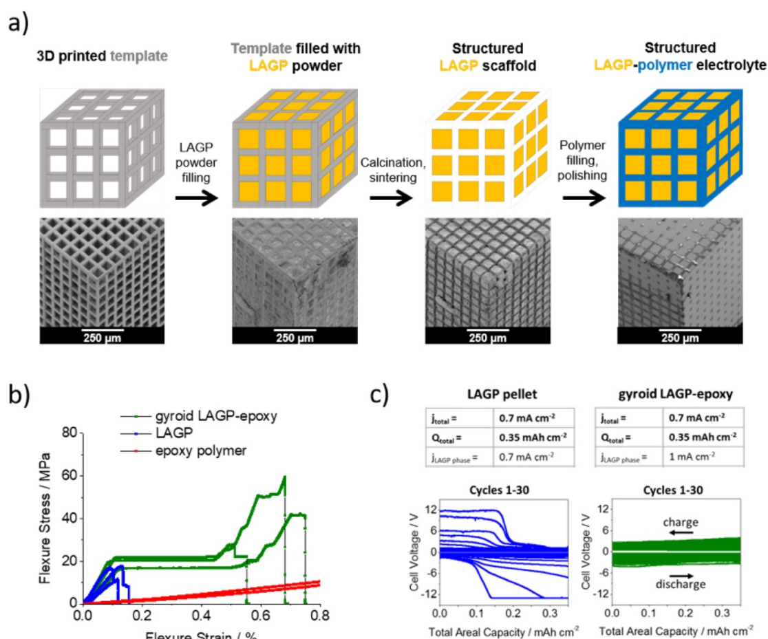
Figure 3. Experimental results showing that increasing the fracture toughness of a solid electrolyte increases critical current density on plating. Schematic and SEM images detailing the preparation of structured ceramics are shown in (a). Hybrid ceramics show a greater fracture toughness (b) and so do not fail at a current density of 0.7 \text{ mA cm}^{-2} whereas non-hybrid ceramics mechanically fracture at this current density. Figure reprinted with permission from [11]. Copyright Energy & Environmental Science.
