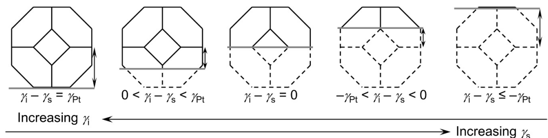
Figure 7. Winterbottom construction for a supported Pt crystal with various degrees of wetting. The grey line represents the substrate. Higher \gamma_i leads to less wetting; higher \gamma_s leads to more wetting. Adapted with permission from [29].
