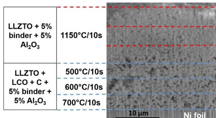
Figure 16. Three spray layers of a composite cathode containing LiCoO 2 (LCO), LLZTO, carbon, solid-state binder and sintering aid Al 2 O 3 , followed by three layers of a LLZTO based electrolyte layer. Each layer was pressureless-sintered for the temperature/time indicated.
