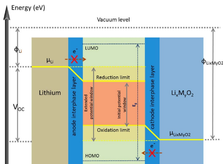
Figure 11. Schematic illustration of open-circuit energy diagram for a solid-state Li-Solid Electrolyte- \text{Li}_x\text{M}_y\text{O}_2 battery. Reprinted with permission from reference [46].
