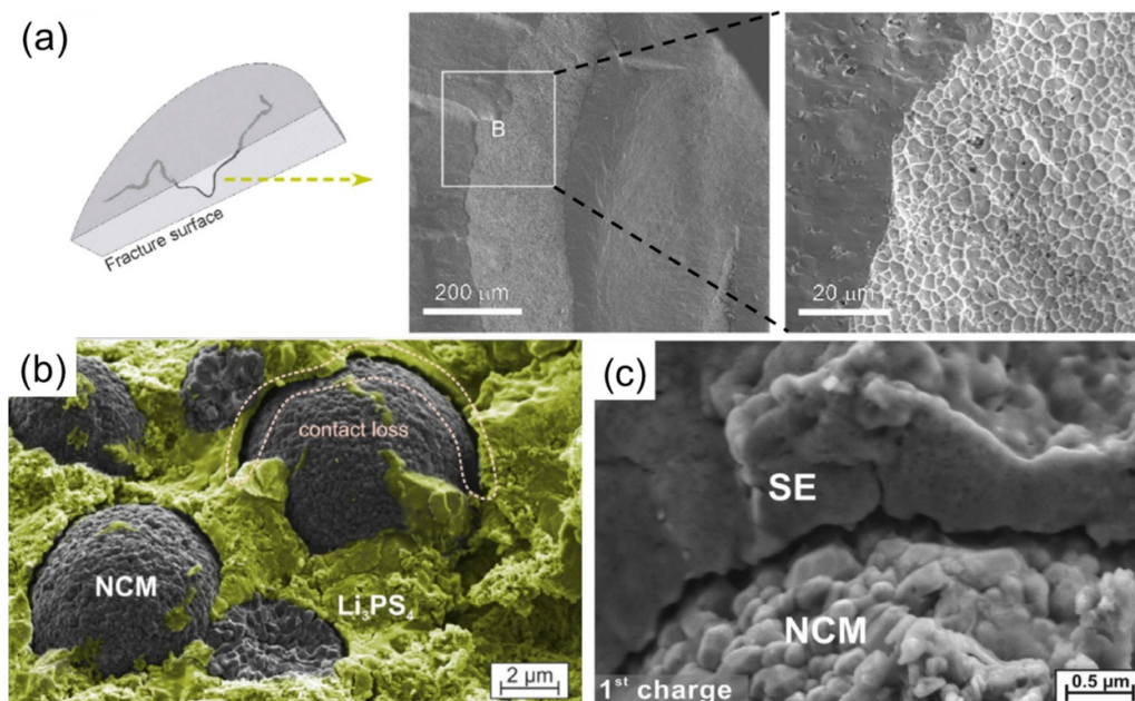
Figure 10. (a) Lithium filament formed in \text{Li}_7\text{La}_3\text{Zr}_2\text{O}_{12} garnet and its microstructure [26]. Reprinted from Electrochimica Acta , 223, Cheng et al , 85–91, Copyright (2017), with permission from Elsevier. (b) Contact loss in NCM-LiPS composite electrodes and (c) details at the NCM-LiPS interface [44]. Reprinted with permission from Chemistry of Materials , 29 (13), 5574–5582, Koerver et al , Copyright (2017), American Chemical Society.
