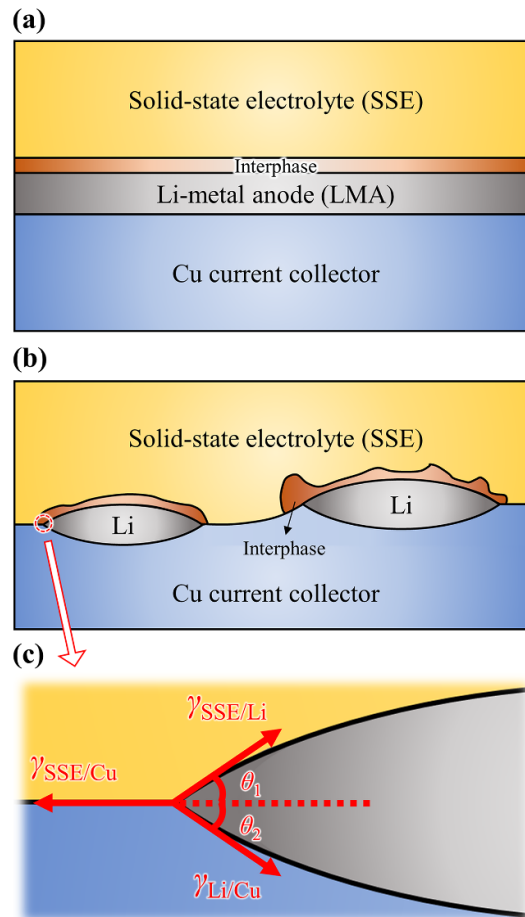
Figure 6. (a), (b) Schematic drawings of two possible interactions between the solid electrolyte (SE), Li-metal anode (LMA), and Cu current collector, and (c) the interfacial energies at a triple junction.
