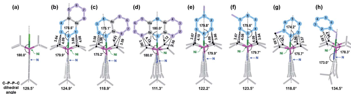
Fig. 4 Top views of optimized structures for (a) (^{acri}PNP)NiCl , 11 (b) 4-Naph , (c) (^{acri}PNP)Ni(1\text{-naphthyl}) , (d) (^{acri}PNP)Ni(9\text{-anthracenyl}) , (e) 4- p Tol , (f) 4- m Tol , (g) 4- o Tol and (h) (^{acri}PNP)Ni(\text{benzyl}) obtained from DFT calculations; distances between atoms in Å.
