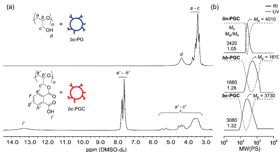
Figure 1. Structural analysis of the obtained topology-controlled polymers: a) 1 H NMR spectra of bc -PG (top) and bc -PGC (bottom); b) RI and UV-SEC curves for the obtained topology-controlled PGCs.
