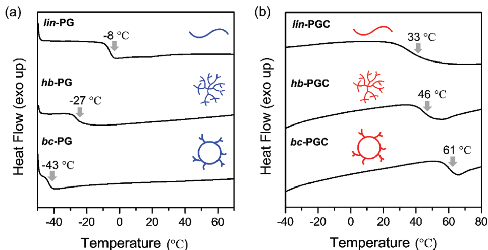
Figure 2. DSC thermograms of the topology-controlled a) PGs and b) PGCs. The 2 nd heating scan is collected at a rate of 10 °C min −1 after heating up to 80 °C.
