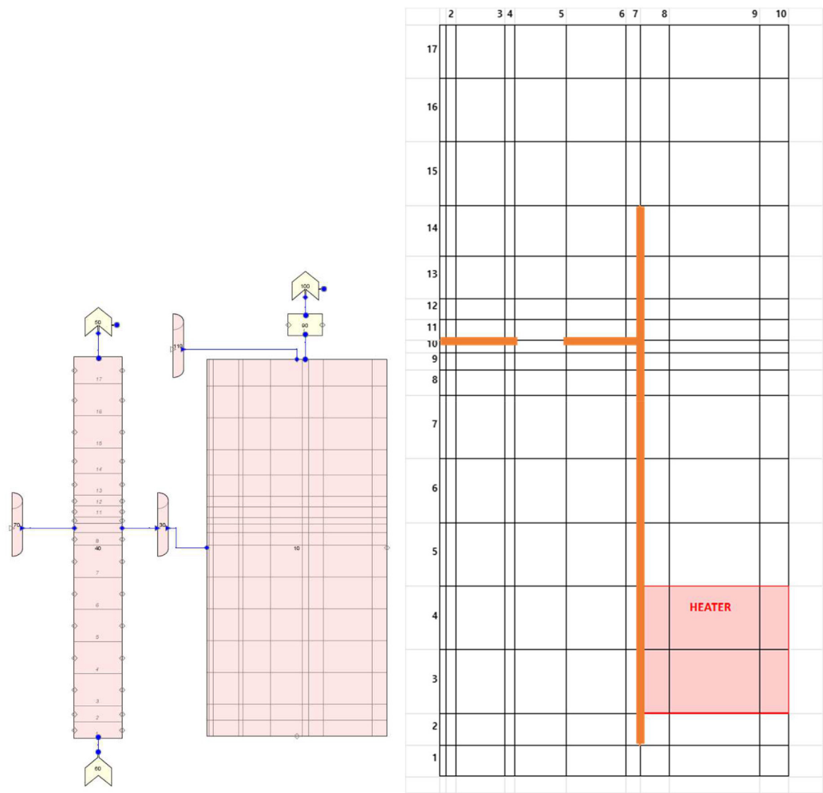
(a) TRACE code nodalization diagram (b) detailed view of the VESSEL component
