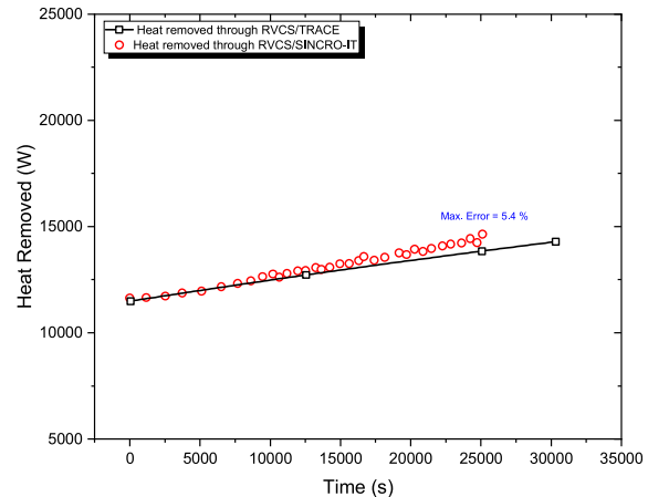
(b) heat removal rate data
