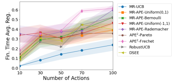
Fig. 3. Effect of number of actions. The time-average final regret \mathcal{R}_T/T at the final round is plotted for different K . All regrets are measured under p = 1.8 and \Delta = 0.7 with Pareto noise distribution. The bold line is an average value of \mathcal{R}_T/T over ten different random seeds and the shaded area indicates a half-standard deviation region.
