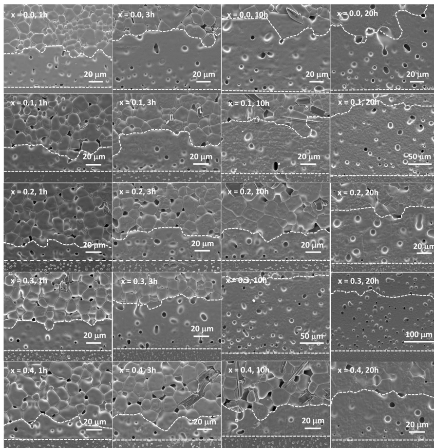
Fig. 6 SEM micrographs of 0.8(\text{Na}_{1/2}\text{Bi}_{1/2})\text{TiO}_3-0.2(\text{Sr}_{1-x}\text{Ca}_x)\text{TiO}_3 single crystals grown on (001) \text{SrTiO}_3 seed crystals at 1200\text{ }^\circ\text{C} for 1, 3, 10, and 20 h.
