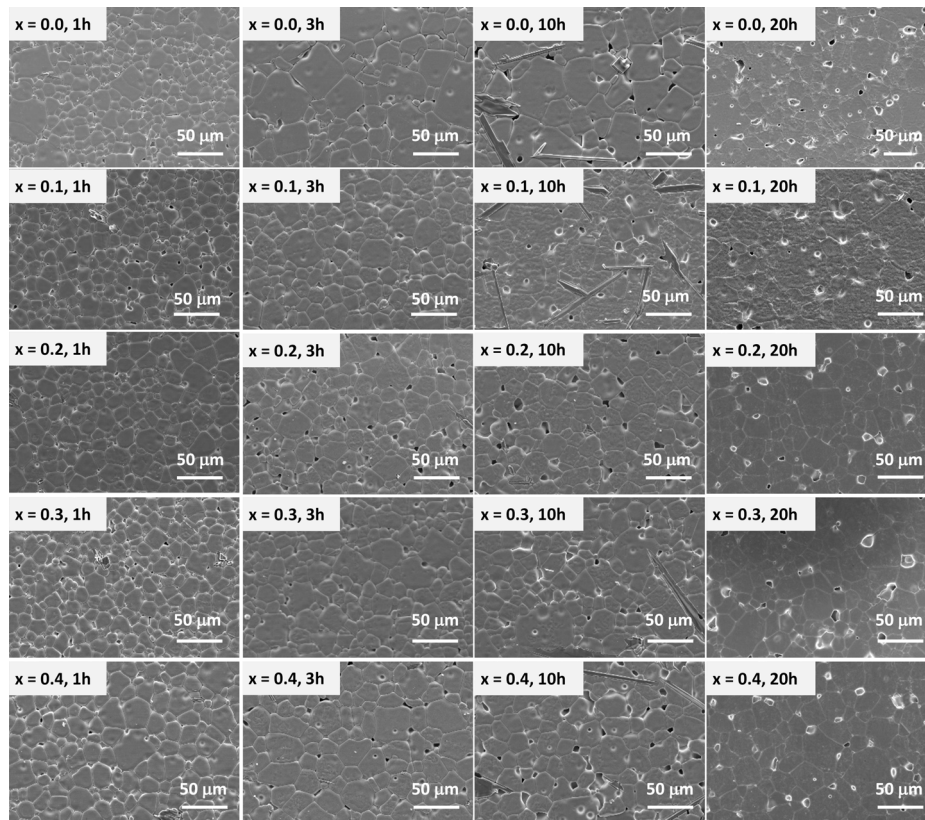
Fig. 8 SEM micrographs of 0.8(\text{Na}_{1/2}\text{Bi}_{1/2})\text{TiO}_3-0.2(\text{Sr}_{1-x}\text{Ca}_x)\text{TiO}_3 matrix grains in samples sintered at 1200 °C for 1, 3, 10, and 20 h.
