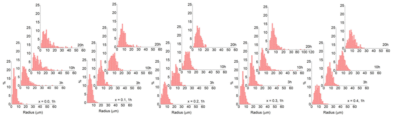
Fig. 9 Matrix grain size distributions of 0.8(\text{Na}_{1/2}\text{Bi}_{1/2})\text{TiO}_3-0.2(\text{Sr}_{1-x}\text{Ca}_x)\text{TiO}_3 samples sintered at 1200 °C for 1, 3, 10, and 20 h. Data for the x = 0.0 composition is taken from Ref. [15].
