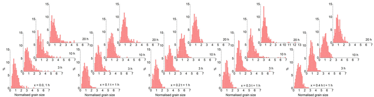
Fig. 10 Normalized matrix grain size distributions of 0.8(\text{Na}_{1/2}\text{Bi}_{1/2})\text{TiO}_3-0.2(\text{Sr}_{1-x}\text{Ca}_x)\text{TiO}_3 samples sintered at 1200 °C for 1, 3, 10, and 20 h. Data for the x = 0.0 composition is taken from Ref. [15].
