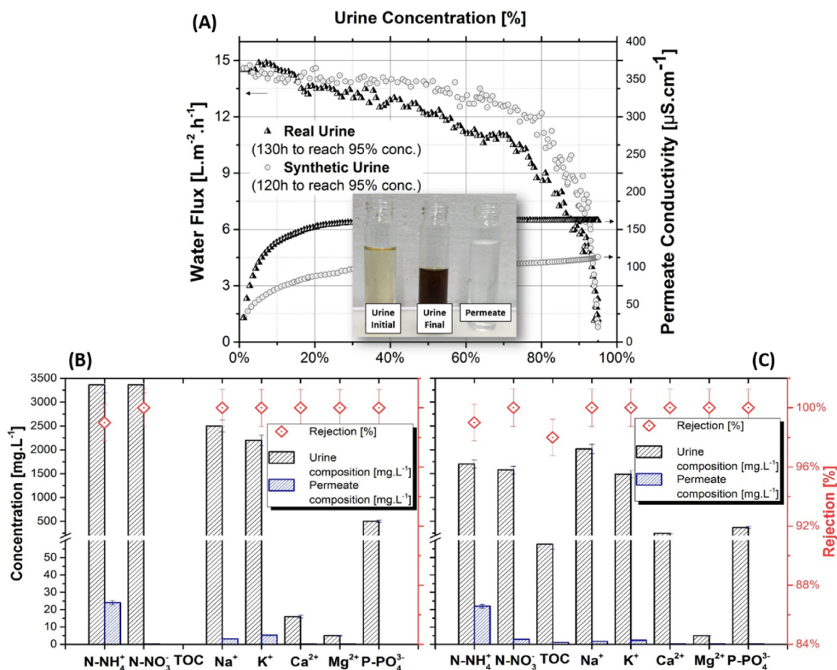
Fig. 4. Above: Permeate flux and electric conductivity of synthetic and real nitrified urine as a function of urine concentration factor ( T_f = 55 \text{ °C} , T_p = 20 \text{ °C} , V_f/p = 0.06 \text{ m s}^{-1} ). Below: Anions, cations and organics concentration in the urine and the final MD permeate using synthetic urine (Fig. B) and real urine (Fig. C). Relative rejection is plotted in red. (For interpretation of the references to colour in this figure legend, the reader is referred to the Web version of this article.)
