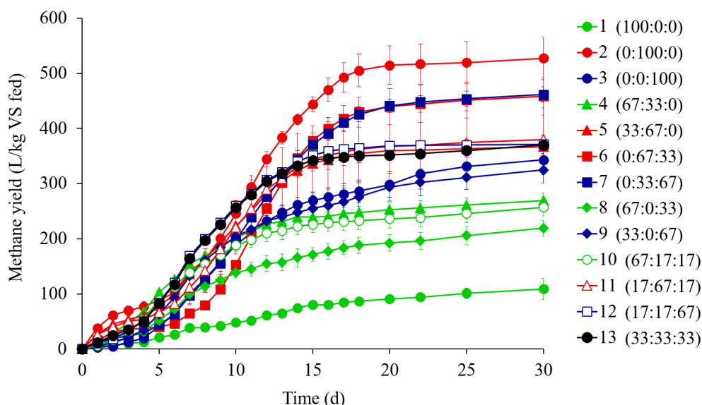
Figure 1. Cumulative methane production in the batch co-digestion tests with cattle manure (CM), food waste (FW), and pig manure (PM). Curves are labeled with the corresponding run numbers (percentage mixing ratio of CM: FW: PM on a total solids basis). Error bars indicate standard deviations ( n = 3 ). Symbol colors represent the composition of substrate mixtures (total solids basis): green for high-CM runs ( \geq 67\% CM), red for high-FW runs ( \geq 67\% FW), blue for high-PM runs ( \geq 67\% PM), and black for the center point run with an equiproportional mixture of CM, FW, and PM.
