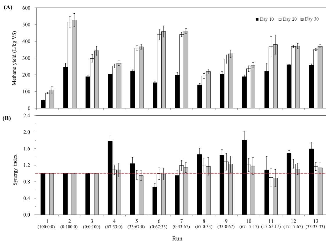
Figure 2. Methane yields (A) and synergy indices (B) determined on days 10, 20, and 30 of the BMP experiments. The CM: FW: PM mixing ratio (total solids basis) for each BMP run is given in parentheses below the corresponding run number. The red dashed line in panel (B) indicates where the synergy index is 1. Error bars indicate standard deviations ( n = 3 ).
