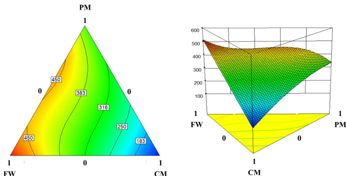
Figure 3. Two- and three-dimensional response surface plots illustrating the effect of the substrate mixing ratio on the 30-day methane yield. Contour colors represent the levels of model response: blue for low and red for high responses.
