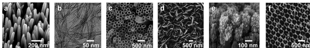
FIG. 2. Electron microscope images of photoanodes based on nanomaterials with various morphologies: (a) ZnO rods, 34 (b) WO 3 wires, 28 (c) TiO 2 tubes, 34 (d) WO 3 plates, 37 (e) \alpha -Fe 2 O 3 dendritic structures, 39 and (f) Bi 2 WO 6 inverse opal. 40 Reproduced by permission from R. H. Gonçalves, L. D. T. Leite, and E. R. Leite, ChemSusChem 5 , 2341 (2012). Copyright 2012 Wiley-VCH. Reproduced by permission from M. Paulose, K. Shankar, S. Yoriya, H. E. Prakasham, O. K. Varghese, G. K. Mor, T. A. Latempa, A. Fitzgerald, and C. A. Grimes, J. Phys. Chem. B 110 , 16179 (2006). Copyright 2006 American Chemical Society. Reproduced by permission from F. Amano, M. Tian, G. Wu, B. Ohtani, and A. Chen, ACS Appl. Mater. Interfaces 3 , 4047 (2011). Copyright 2011 American Chemical Society. Reproduced by permission from A. Kay, I. Cesar, and M. Gratzel, J. Am. Chem. Soc. 128 , 15714 (2006). Copyright 2006 American Chemical Society. Reproduced by permission from L. W. Zhang, C. Baumanis, L. Robben, T. Kandiel, and D. Bahnemann, Small 7 , 2714 (2011). Copyright 2011 Wiley-VCH.
