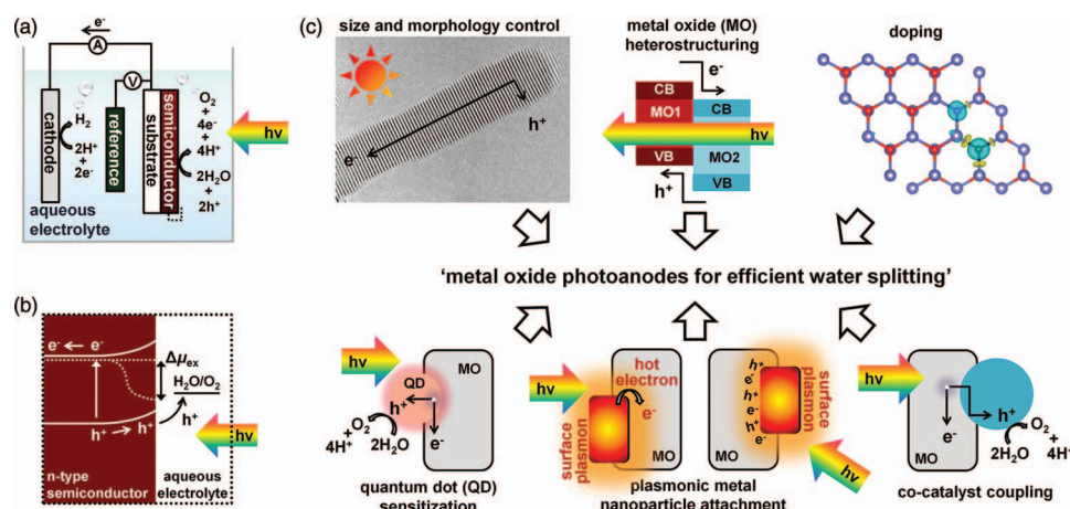
FIG. 1. (a) Schematic diagram of a photoelectrochemical water splitting cell. (b) Electron energy scheme of a n-type semiconductor in an aqueous electrolyte. (c) Strategies for efficient metal oxide photoanodes.
