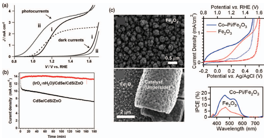
FIG. 5. (a) Current-potential curves of \alpha\text{-Fe}_2\text{O}_3 photoanodes (i) before and (ii) after \text{IrO}_2 coupling. 121 Reproduced by permission from S. D. Tilley, M. Cornuz, K. Sivula, and M. Gratzel, Angew. Chem., Int. Ed. 49 , 6405 (2010). Copyright 2010 Wiley-VCH. (b) Chronoamperometry for \text{CdSe/CdS/ZnO} nanowire electrode before and after \text{IrO}_x \cdot n\text{H}_2\text{O} modification, at 0.6 V (vs. RHE) under 1 sun simulated AM1.5 illumination. 122 Reproduced by permission from M. Seol, J. W. Jang, S. Cho, J. S. Lee, and K. Yong, Chem. Mater. 25 , 184 (2013). Copyright 2013 American Chemical Society. (c) SEM images, dark (dashed) and photocurrent (solid) densities and incident photon-to-current conversion efficiency spectra of mesostructured \alpha\text{-Fe}_2\text{O}_3 photoanodes before and after electrodeposition of cobalt phosphate. 128 Reproduced by permission from D. K. Zhong, J. W. Sun, H. Inumaru, and D. R. Gamelin, J. Am. Chem. Soc. 131 , 6086 (2009). Copyright 2009 American Chemical Society.
