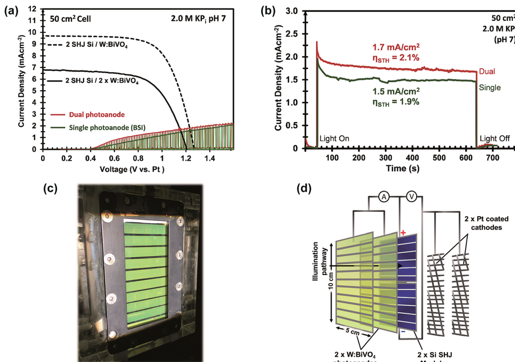
Fig. 8 (a) J - V curves for the 50\text{ cm}^2 2 \times SHJ PV module behind single (dashed black lines) or dual (solid black lines) \text{W:BiVO}_4 photoanodes, and J - V curves for the 50\text{ cm}^2 single (green) and dual (red) \text{W:BiVO}_4/\text{CoP}_i photoanodes under chopped AM 1.5G illumination. (b) Current density and voltage vs. time for the 50\text{ cm}^2 PEC-PV devices with single (green) and dual (red) photoanode configurations over 10 min. All measurements were conducted in a stirred 2.0\text{ M KPi} electrolyte at pH 7. (c) Photograph of the large area ( 50\text{ cm}^2 ) integrated PEC-PV device in the dual photoanode configuration with a device structure of \text{W:BiVO}_4(\text{BSI})/\text{Electrolyte}/\text{W:BiVO}_4(\text{FSI})/2\text{SHJ-PV}/2\text{Pt} , illustrated in (d). BSI: back-side illuminated, FSI: front-side illuminated.
