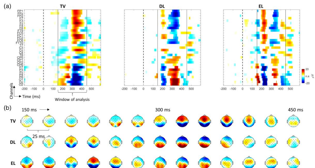
Figure 3. (a) Time-channel ERP maps and (b) topological map of scalp. Color scale denotes significantly different ERP amplitude by the two-sample t -test on a sample-by-sample basis ( p < 0.01 ). (a) The vertical solid dark lines denote the window of analysis from 150 to 450 ms. (b) An individual topological map indicates a time instant within the window of analysis, which is represented as the interval of 25 ms.
