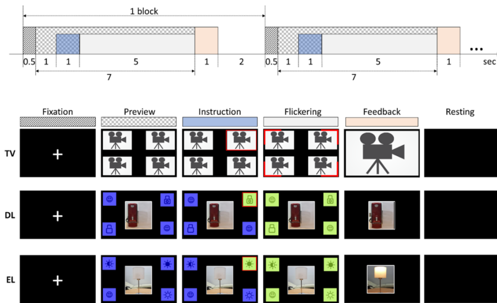
Figure 1. Experimental paradigm and stimulus sequence for each device control. (Top panel) Task protocol for each block. One block implies selecting one target at once. (Bottom panel) Stimulus sequence for each device; TV, DL (door lock), and EL (electric light).
