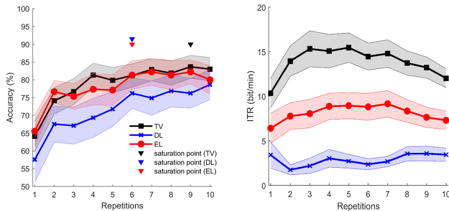
Figure 5. Performance changes depending on the number of stimulation repetitions. (Left panel) Shows the curves of classification accuracy of each type of BCIs. (Right panel) shows those of the information transfer rate (ITR).
