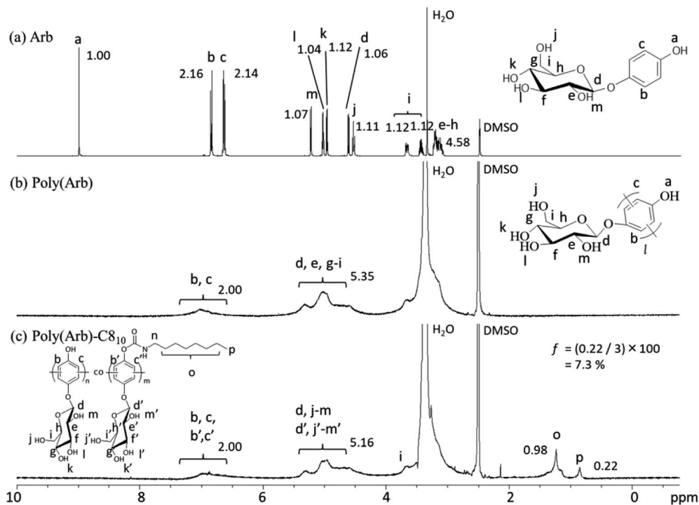
Fig. 1 1 H NMR spectra of (a) Arb, (b) poly(Arb), and (c) poly(Arb)-C8 10 in DMSO- d 6 .
