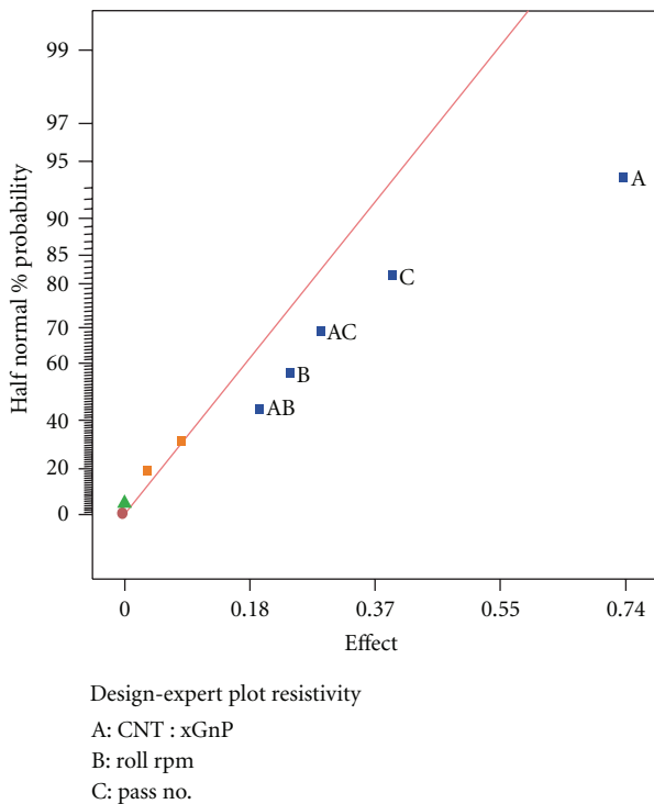
FIGURE 3: Half normal plot.
