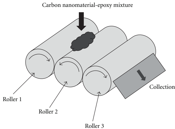
FIGURE 1: Schematic of three-roll mill.
