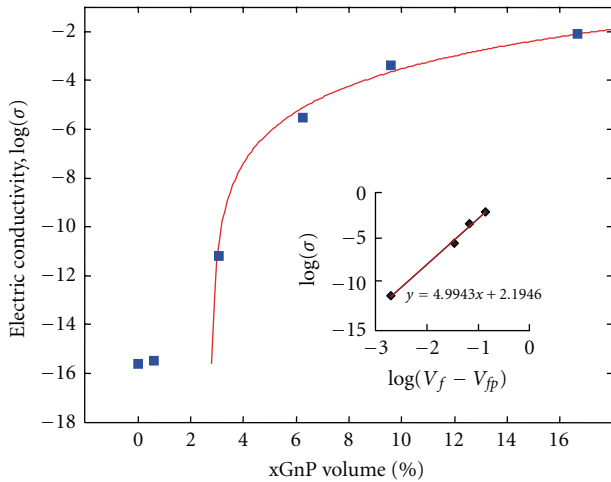
FIGURE 2: Measured and predicted electrical conductivities of xGnP-epoxy composites.
