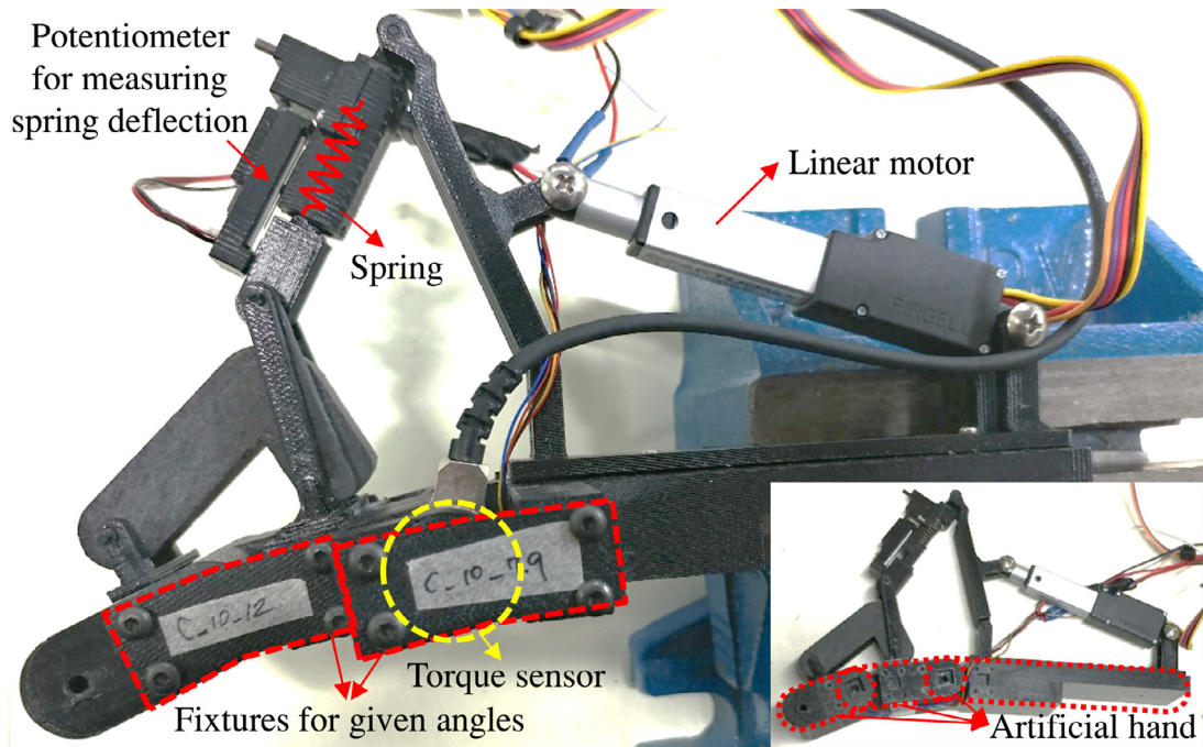
Fig. 14. Experimental setup.
