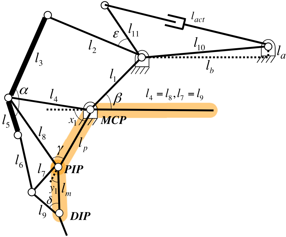
Fig. 6. Parameters considered when designing the exoskeleton system.
