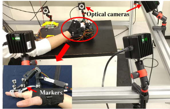
Fig. 12. Experimental setup.
