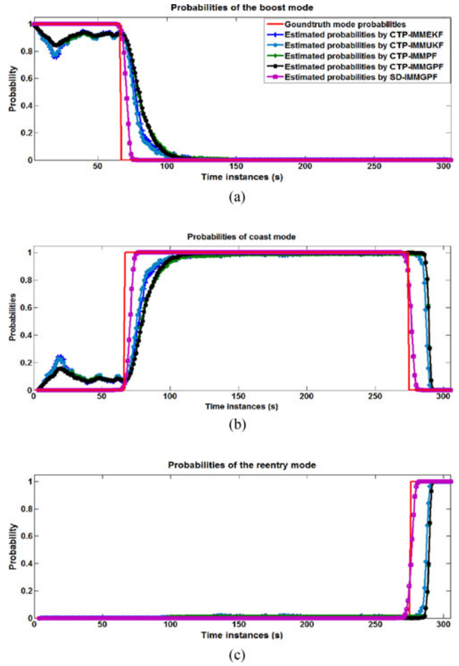
Fig. 6. Estimated flight phases probabilities by different estimation algorithms. (a) Boost phase. (b) Coast phase. (c) Reentry phase.
