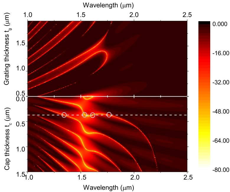
Fig. 4. Contour plot of transmissivity in dB as a function of wavelength, grating thickness, t_g , and cap layer thickness, t_c . In the upper graph, t_g is increased from 0.497 \mu\text{m} to 1.997 \mu\text{m} while t_c is zero. In the lower graph, t_c is increased from 0 to 1.5 \mu\text{m} while t_g is kept to 0.497 \mu\text{m} . The white dashed line shows the cap layer thickness of the HG structure considered in Fig. 2 and the circles indicate the wavelengths of the four GMRs.
