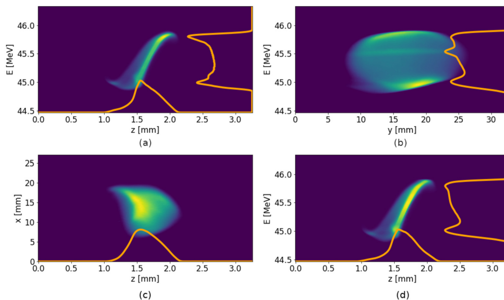
Fig. 9. (a to c) Experimental YAG images taken with the wiggler out of the beamline, in the case of the round beam. All images show a bunch with charge Q = (300 \pm 4) pC. (a) LPS observed on YAG6 with the TDC and spectrometer turned on. For this image a horizontal slit was placed in front of the TDC. (b) Energy distribution of the beam observed on YAG6, obtained with the spectrometer turned on. (c) Longitudinal particle distribution observed on YAG5 with the TDC turned on. (d) Numerical particle distribution generated by combining images a, b and c, which was used for the back-tracking simulations.
