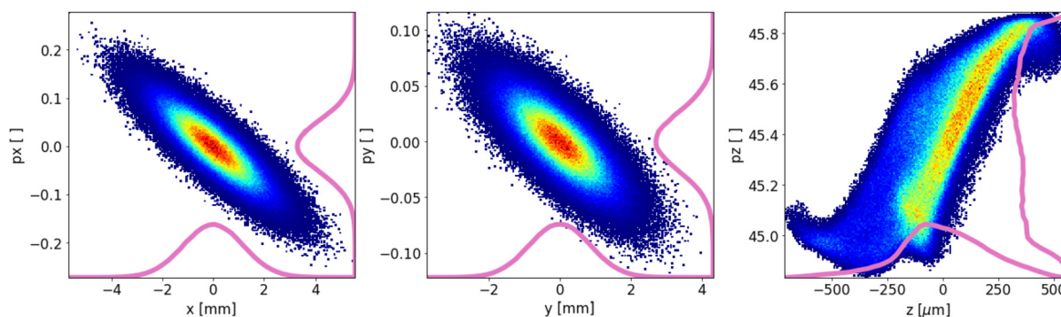
Fig. 10. Initial particle distribution for the simulations of the round beam. This is the bunch's 6D phase space at YAG1.
