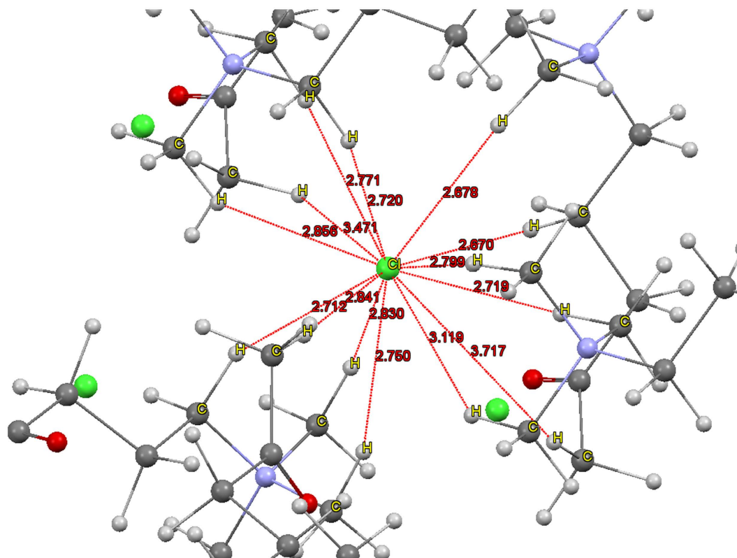
Figure 3. Fourteen C–H...Cl − interaction sites in crystal structures of BUXTOD systems 39 , where only H positions were optimized at the B97D/cc-pVDZ level. The direct Cl − ...C binding distances (Å) are denoted in red color (green: Cl − , blue: N, red: O, dark gray: C, light gray: H).
